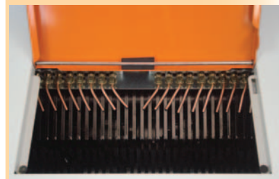
Optional EvenFlow™ Oiling System heavy-duty copper nozzles
